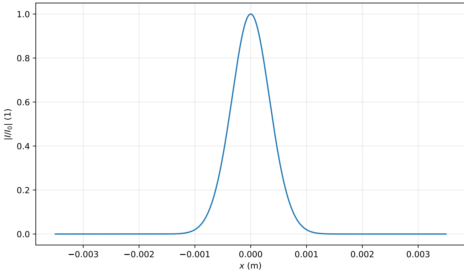
Intensity profile I(x, y = 0, z = 0.478m)/I_0 , \text{Pin}=0.3\text{Pcr} , artificial time
